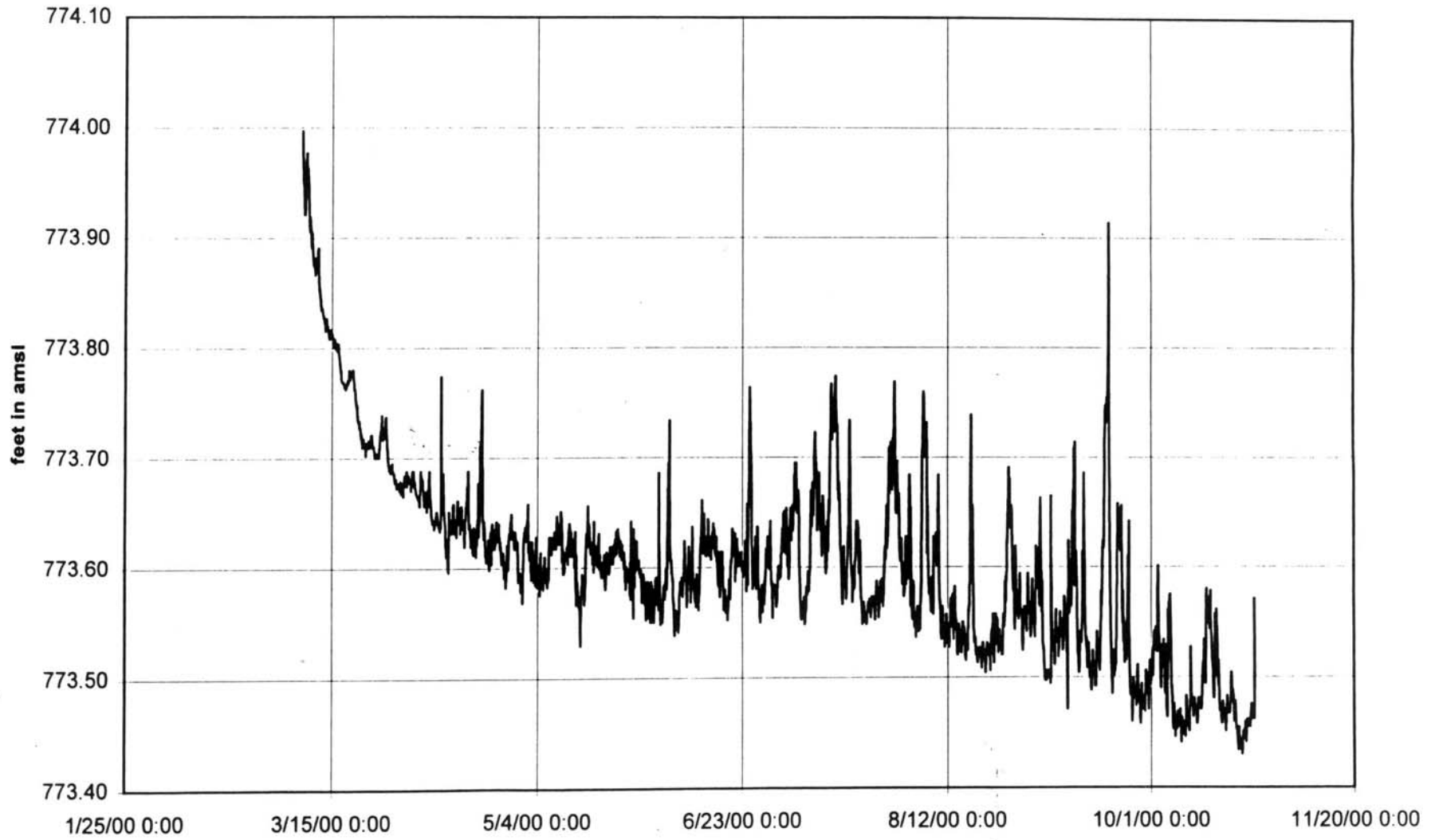
Figure 2 Neals Landfill Piezometer 01 Data for 2000
