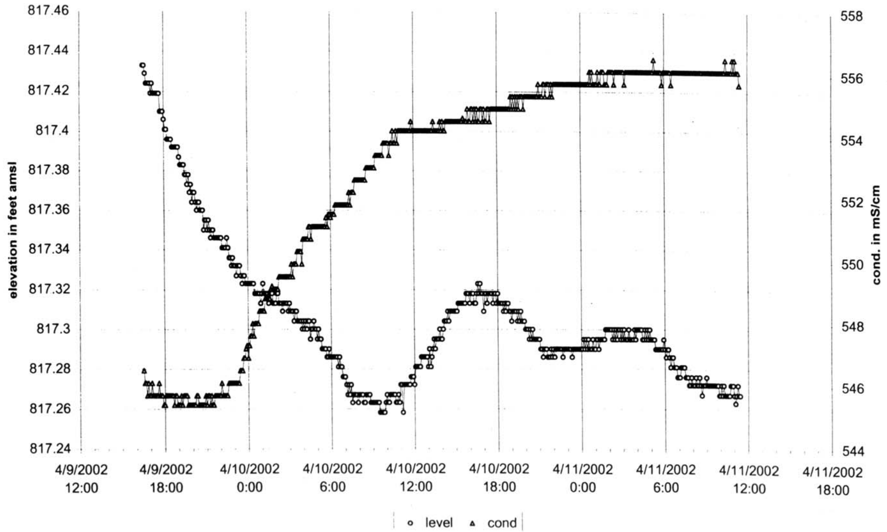
Figure 1A Water Elevation and Conductivity in MW-21 During LF6 Flood Test
